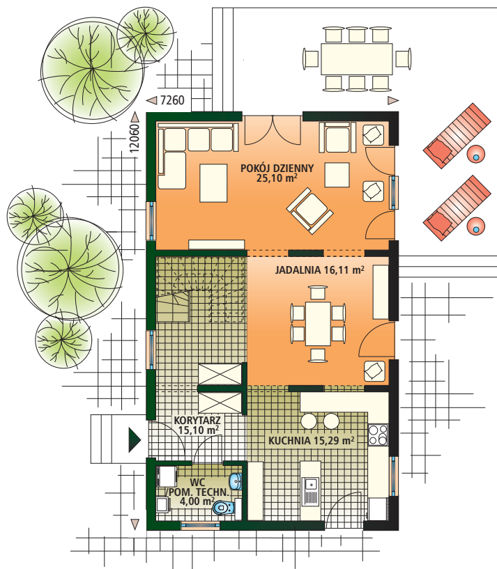
PARTER 75,60 m 2
